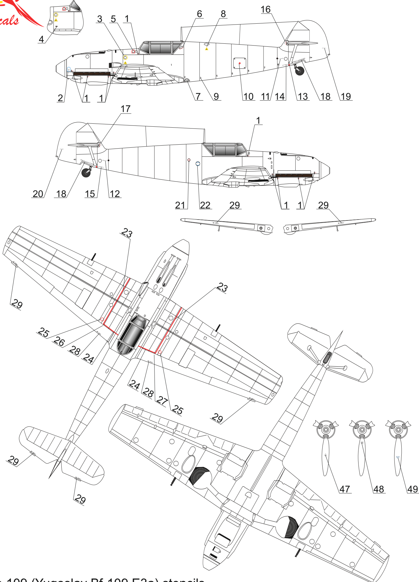
Me 109 (Yugoslav Bf-109 E3a) stencils
